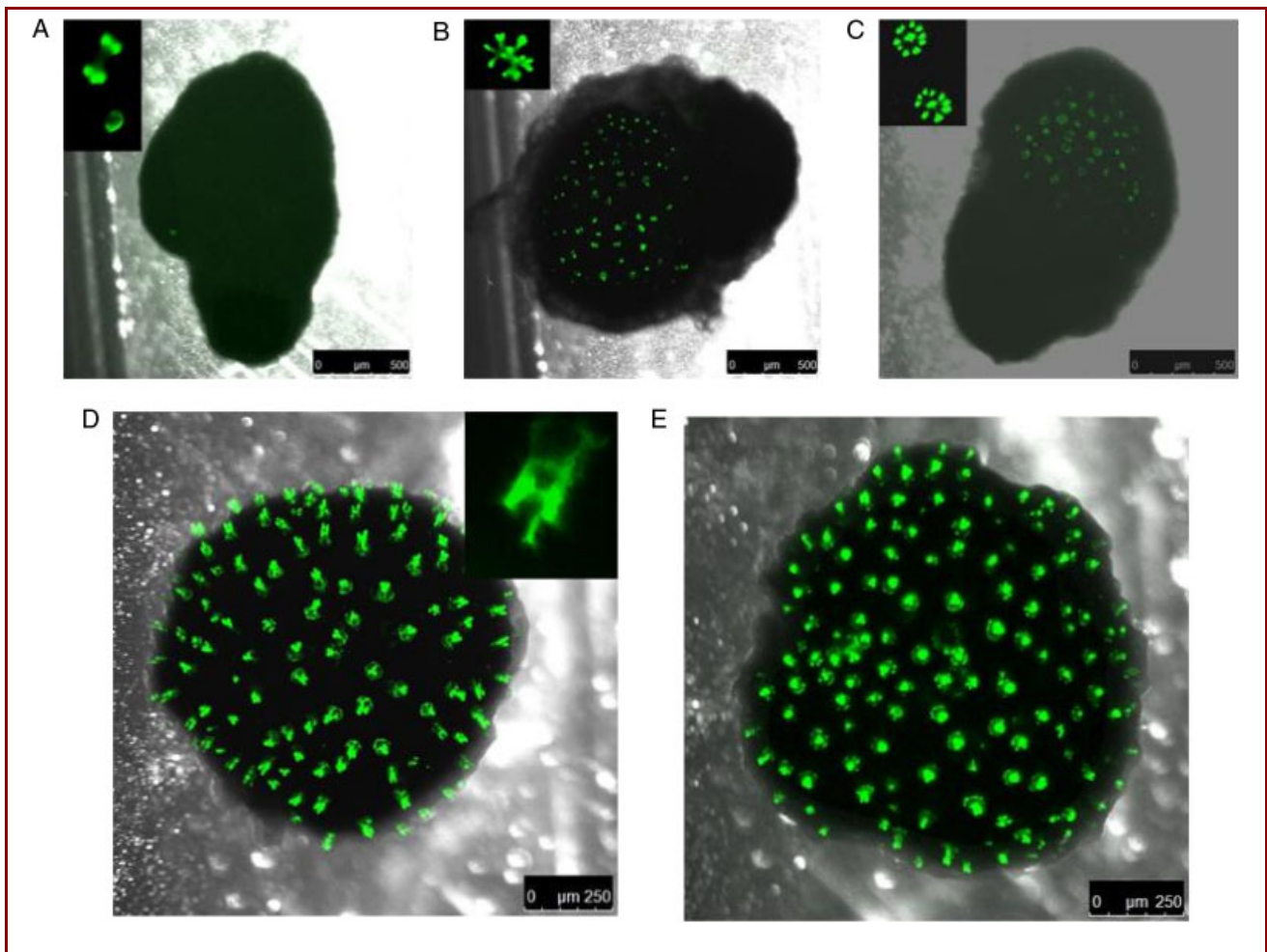
Figure 3. Confocal image of calcein-labeled skeleton during development of C. papposus . (A) (pH 8.1, d7): small isolated crystals are the first sign of calcification; (B) (pH 7.7, d7) and (C) (pH 8.1, d24) crystals are more complex and widespread on all the aboral surface; (D) (pH 7.7, d28) and (E) (pH 8.1, d38): well-developed spines are visible after 28d in acidic conditions and more developed than in the control after 38 days.
