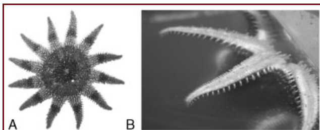
Figure 1. (A) Specimen of Crossaster papposus . (B) Female naturally spawning in the aquarium. The large yolky red eggs are visible floating on the surface of the aquarium.
