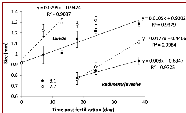
Figure 5. Growth of larvae and juveniles of the starfish C. papposus under controlled (pH 8.1) and near-future acidic conditions (pH 7.7 expected for 2100). Under acidic conditions, growth rates are two times higher.
