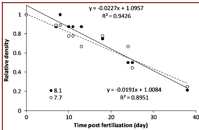
Figure 4. Density of larvae and juveniles of the starfish C. papposus under control (pH 8.1) and near-future acidic conditions (pH 7.7 expected for 2100). No difference was observed between the treatments.
